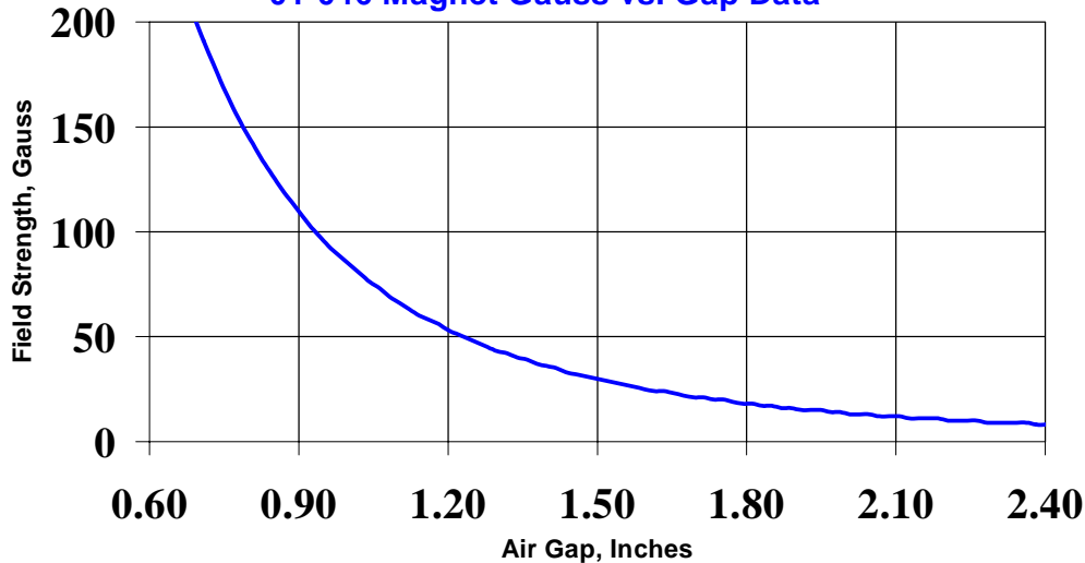
01-046 Magnet Gauss vs. Gap Data
