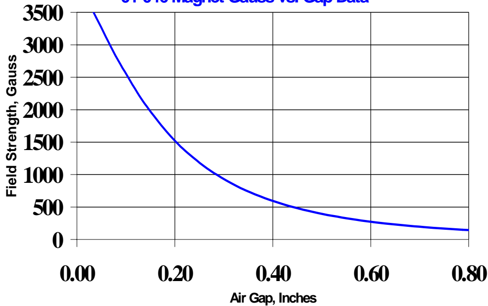
01-046 Magnet Gauss vs. Gap Data
